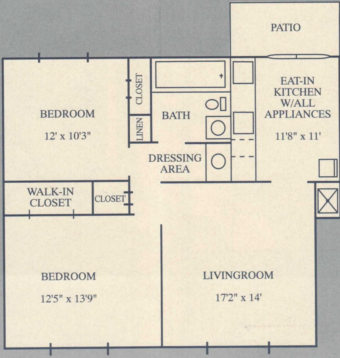
Typical Floorplan
